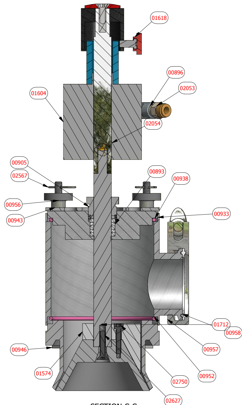
SECTION C-C SCALE 1/2
